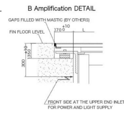
B Amplification DETAIL
