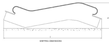
SHIPPING DIMENSIONS
